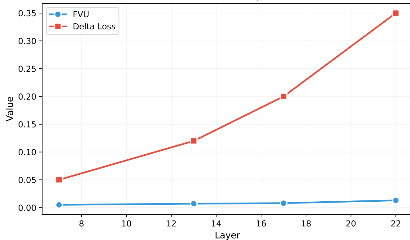
FVU Stays Low While Delta Loss Grows with Depth
